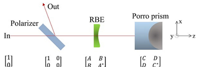
Figure 18 Schematic diagram of the orthopedic system and Jones matrix
