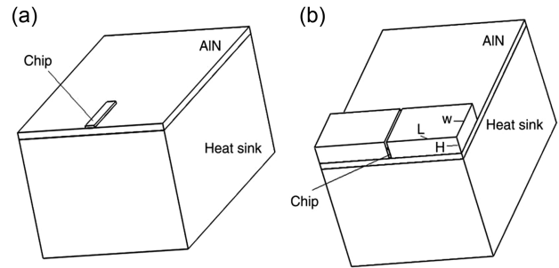
Figure 5 Traditional and new structures
