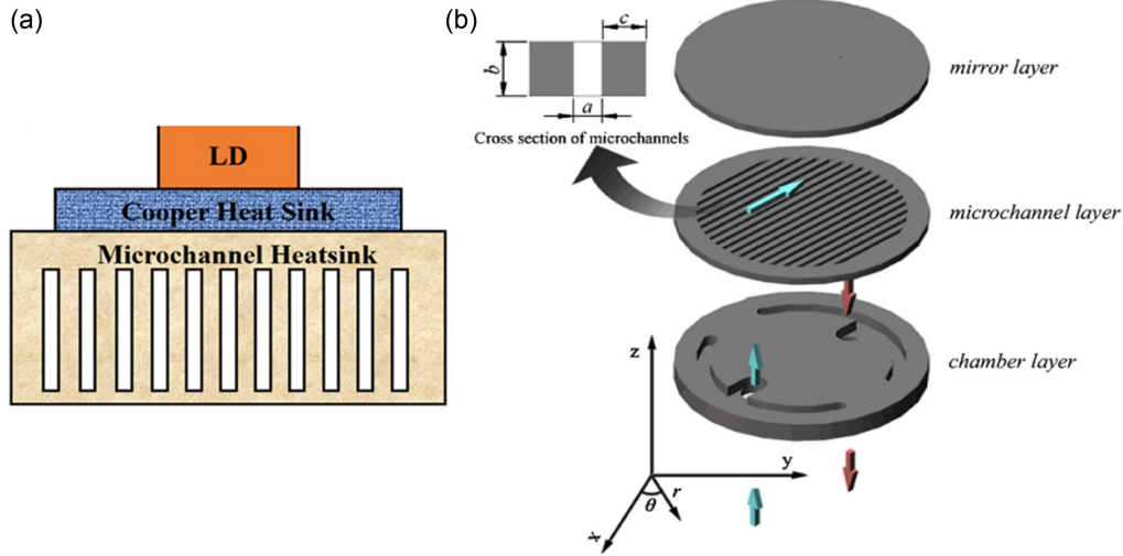
Figure 3 (a) Typical microchannel heat sink structure (b) Some kind of microchannel heat sink profile
