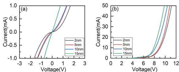
FIG. 4. (a) Current–voltage (I–V) curves with different V thicknesses in the same gap of 10- \mu\text{m} . (b) Current–voltage (I–V) characteristics after device fabrication. The smaller the intercept, the better the ohmic contact.
